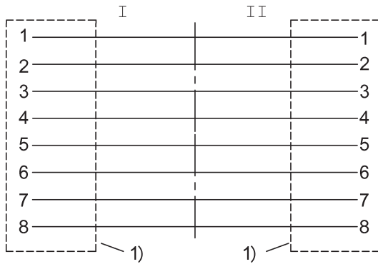
1) Shielded knurl
