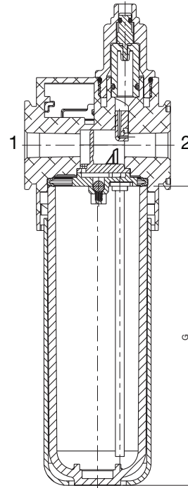
Cross Section - 651/652/653 Series Lubricator
