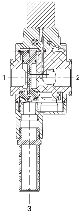
Cross Section - 651/652/653 Series Slow Start/Quick Exhaust Valve
